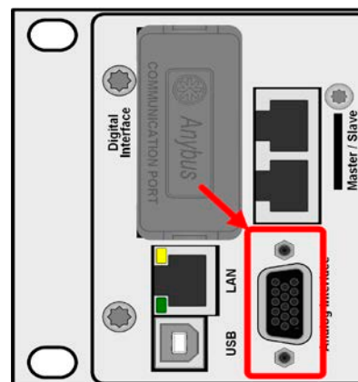
Figure 4 - Interface analogique
