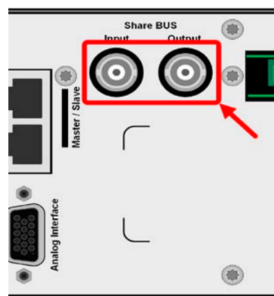
Figure 5 - Share bus
