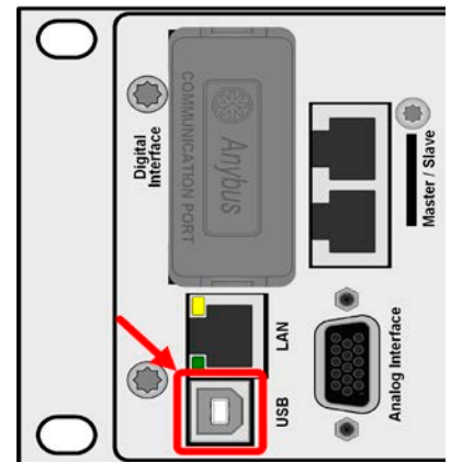
Figure 2 - Port USB
