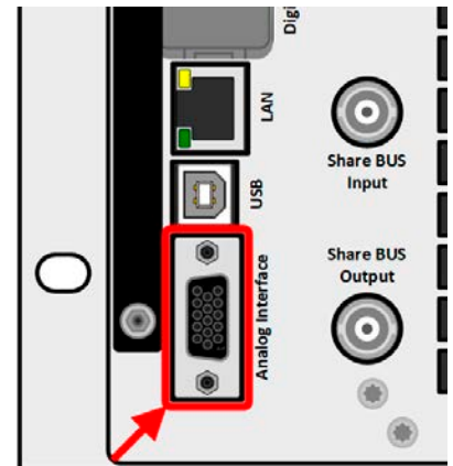
Figure 4 - Interface analogique
